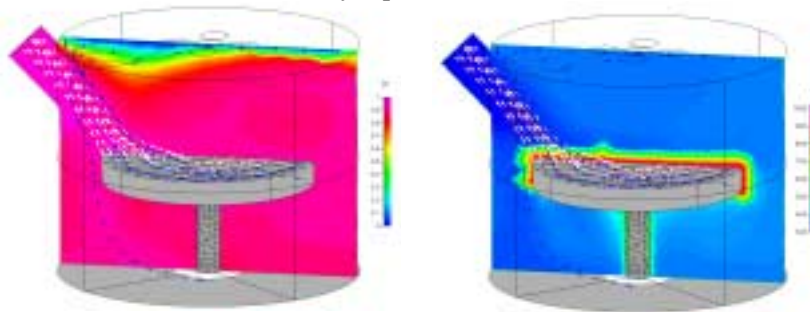
(e) Purge gas molar concentration distribution, (f) Temperature distribution Port flow density 10x uniform flowrate.
