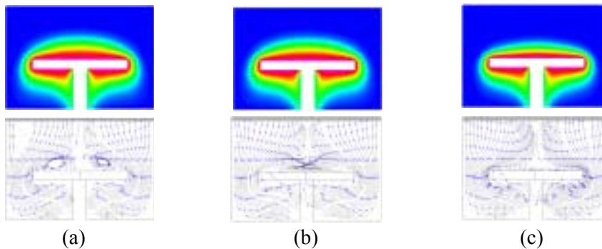
Figure 4. Simple comparison of rotation effects on a 5'' platter operated at 20 Torr and (a) 0 rpm, (b) 200 rpm, and (c) 750 rpm.
