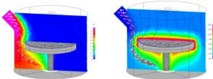
(c) Purge gas molar concentration distribution, (d) Temperature distribution Port flow density equal to the uniform flux.
