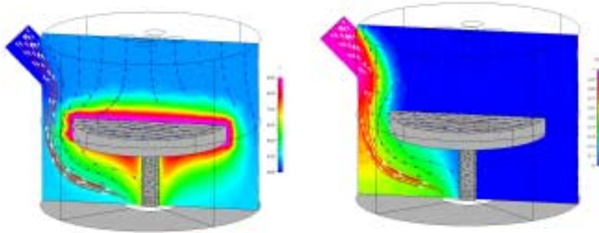
(a) Temperature distribution, (b) Purge gas molar concentration distribution Port flow density is 1-% of the uniform flow.
