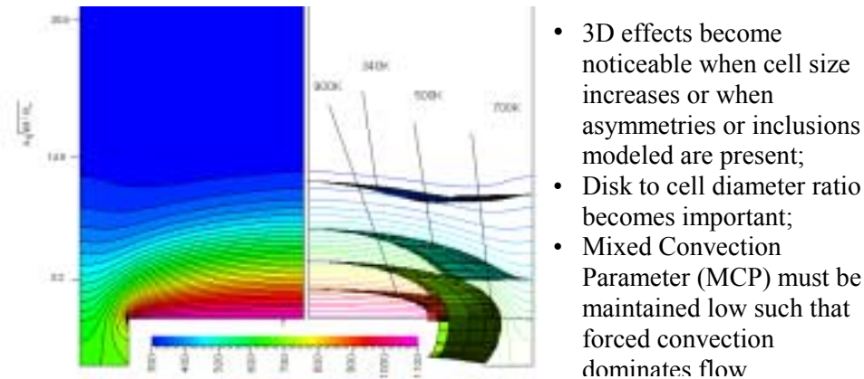
Figure 3. Comparison of results for 2D and 3D.
