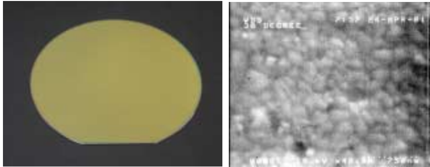
Figure 17. (a) Photograph of a Spin CVD PZT film deposited on a 6” wafer, showing a uniform color, and (b) SEM microphotograph of an equivalent film, highlighting the grain structure achieved.
